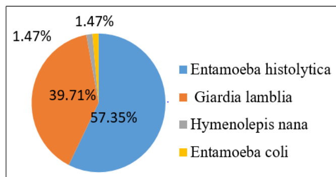
Fig. 2: Parasite Wise Distribution of Intestinal Parasites
