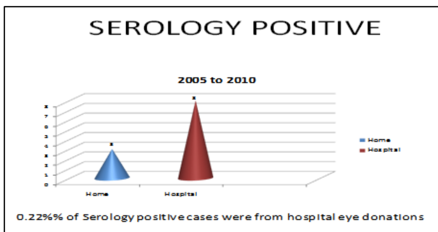
Figure 9. Serology Positive
